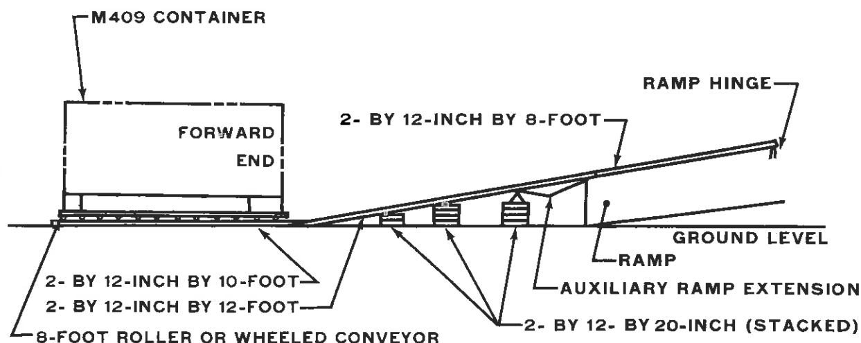
Figure 4-2. Side view schematic of rolling and blocking shoring positioned for loading Nike-Hercules warhead section shipping and storage container, M409, into CH-47 helicopter.
