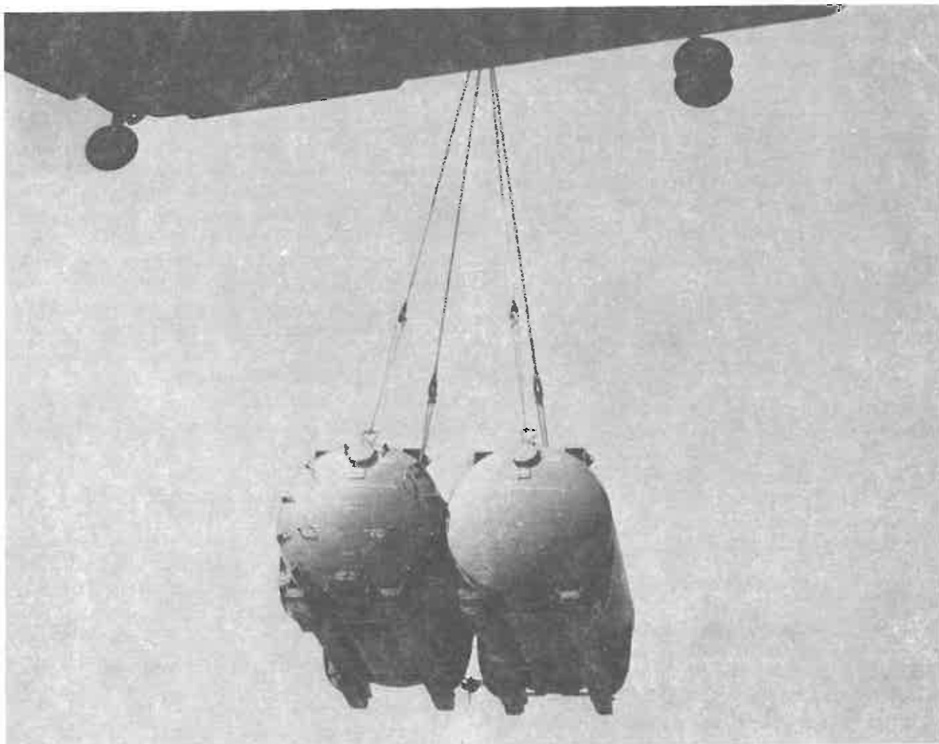
Figure 4-11. External transport of two Nike-Hercules warhead section containers, M409. Containers are lashed together at both ends by chains between the tiedown bars.
