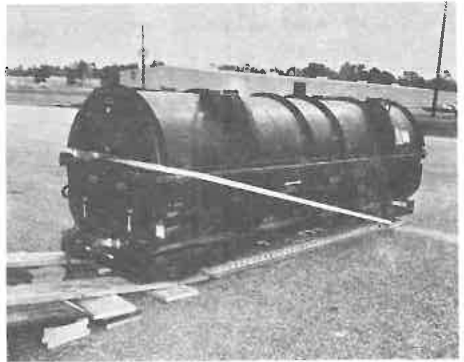
Figure 4-5. Placement of CGU-1/B tiedown devices to restrain container during loading. Shown is the M483 container for Pershing warhead section.
