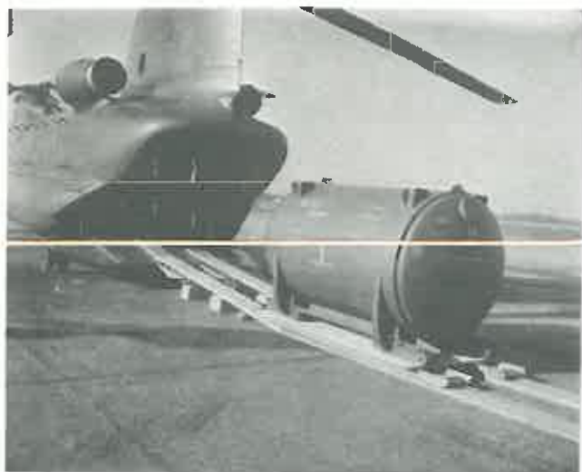
Figure 3-1. Shipping and storage container, M409, for Nike-Hercules warhead section. Container is positioned for loading into CH-47 helicopter.
